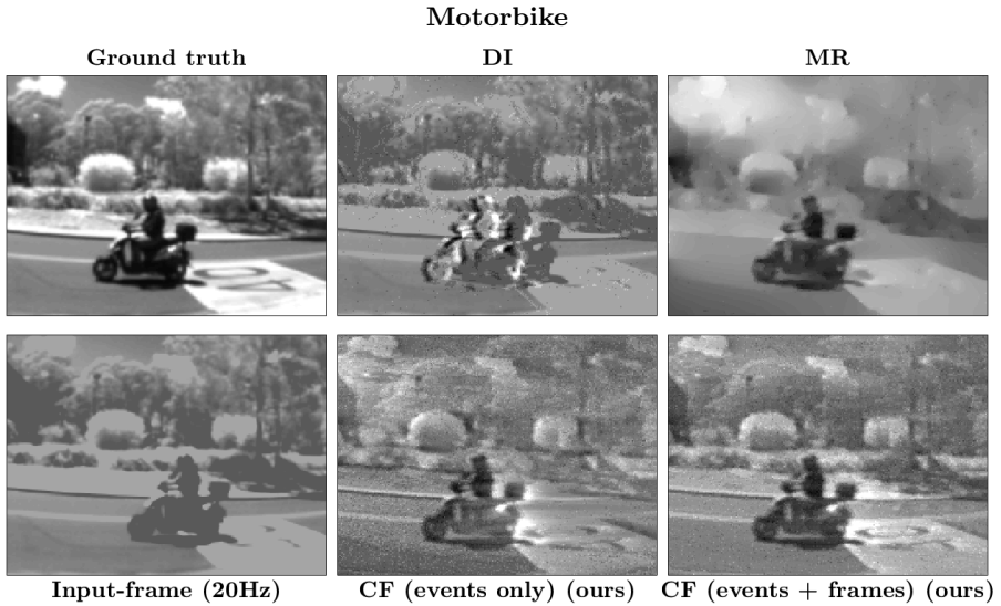
Fig. 2. CF shows good resemblance to ground truth despite added noise in the event-stream, and temporally sparse, lagged, low-dynamic-range input-frames. DI displays separation of moving objects between input-frames and event information. MR tends to over-smooth the background, which generates fewer events than the foreground.
