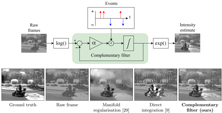
Fig. 1. The complementary filter takes image frames and events, and produces a high-dynamic-range, high-temporal-resolution, continuous-time intensity estimate.
