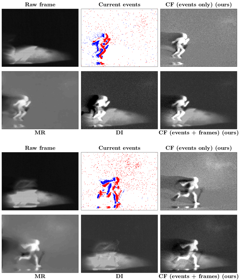
Fig. 4. Night run sequence. The frame-based camera produces a lagged, heavily motion blurred image. DI is adversely impacted by every reset (bottom). The high temporal resolution of the event camera allows sharp reconstruction of person running quickly (MR and CF). CF (events + frames) is additionally able to capture the area of the road lit by the headlights.
