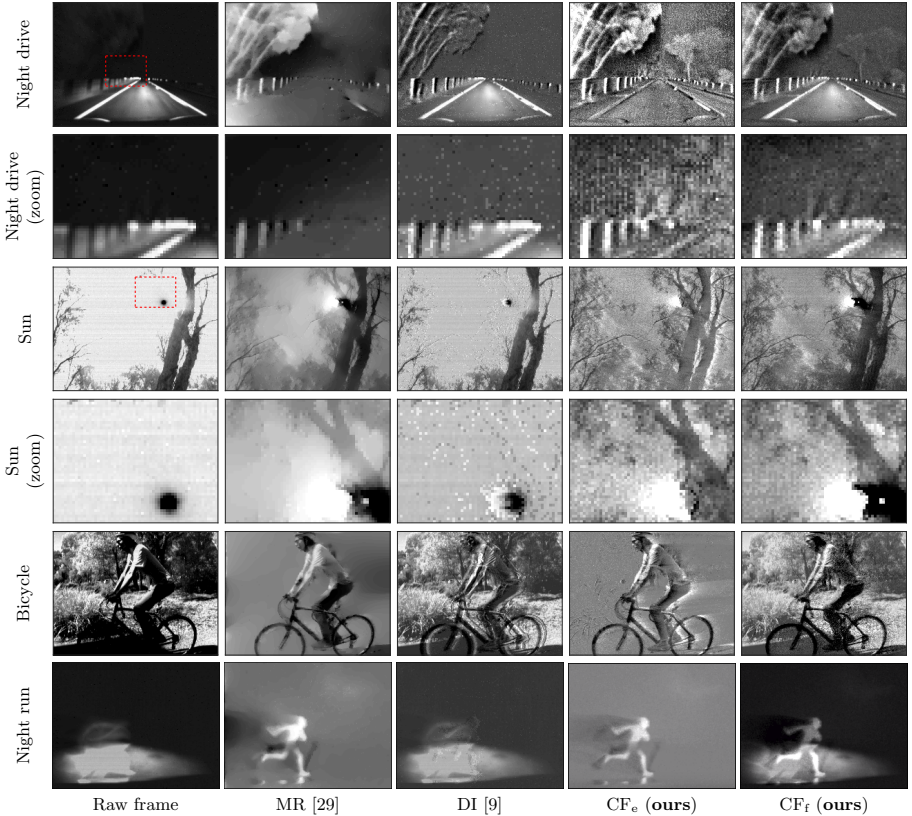
Fig. 2. Night drive: Raw frame is motion-blurred and contains little information in dark areas, but captures road markings. MR is unable to recover some road markings. CF_f recovers sharp road markings, trees and roadside poles. Sun: Raw frame is overexposed when pointing directly at the sun (black dot is a camera artifact caused by the sun). In MR, some features are smoothed out (see zoom). DI is washed out due to the latest frame reset. CF captures detailed leaves and twigs. Bicycle: Static background cannot be recovered from events alone in MR and CF_e . CF_f recovers both background and foreground. Night run: Pedestrian is heavily motion-blurred and delayed in Raw frame. DI may be compromised by frame-resets. MR and CF recover sharp detail despite high-speed, low-light conditions.
