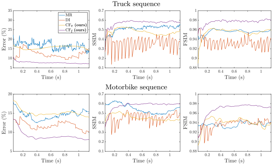
Fig. 3. Full-reference quantitative evaluation of each reconstruction method on our ground truth datasets using photometric error (%), SSIM [33] and FSIM [34].
